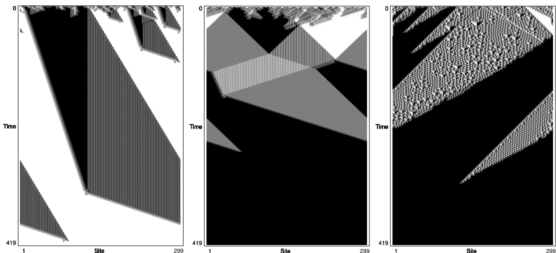
Figure 6.6: GA evolved rules for one-dimensional density classification task. The rules were found by Das et al. (left)[28], Marques-Pita (center)[79, 83] and Wolz & de Oliveira (right)[140].
