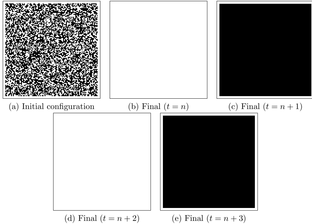
Figure 3.3: Example of a Global Synchronization task. (a) Sample IC representing the initial state of the processors, while (b) - (e) show the desired output as an alternation of all processors On (all white) and Off (all black) configuration.
