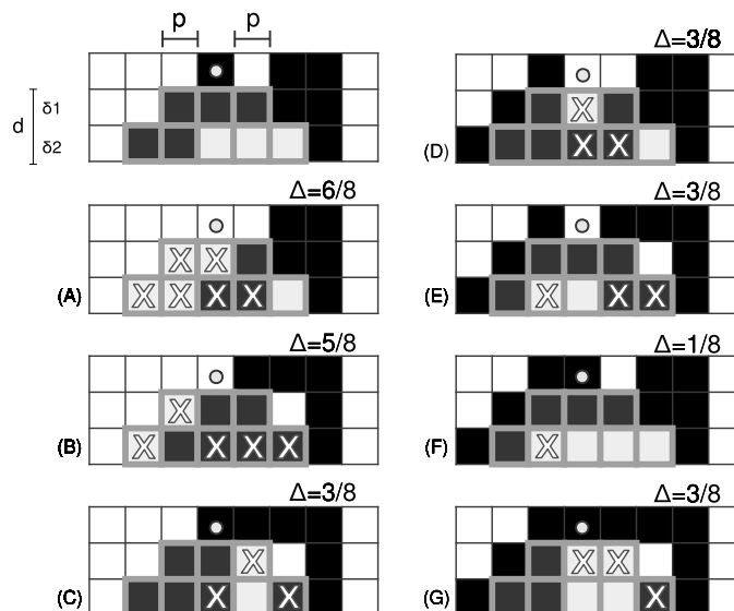
Figure 7.6: Example of the calculation of \xi_2^1(4,0) . The top-left corner shows the original initial configuration and two updates using elementary CA 110. The local sensitivity is calculated for the fourth site at time t = 0 (highlighted with a circle). The perturbation range is p = 1 , which determines the perturbation neighborhood P = \langle 0, 1, 0 \rangle , and the future depth is set to d = 2 . The sites that depend on the information stored in site (4,0) (for a 1D radius r = 1 CA, within future-depth 2) are marked with grey squares. They determine the future light-cone for (4,0) . The perturbation neighborhood P generates |S| = 7 “words” of length three. Diagrams (A)–(G) show the behavior of the CA when each of these words replaces the original configuration in the perturbation range, and the CA is run for d = 2 time steps. The cells in each future light-cone that differ from the corresponding cells in the original future light-cone are marked with an X . The Hamming distance \Delta , i.e., the fraction of differing cells between the original future light-cone and the one resulting from each perturbation is shown above the top-right of each diagram in (A)–(G). These seven \Delta ’s are averaged, resulting in a local sensitivity \xi_2^1(4,0) = 0.4285 .
