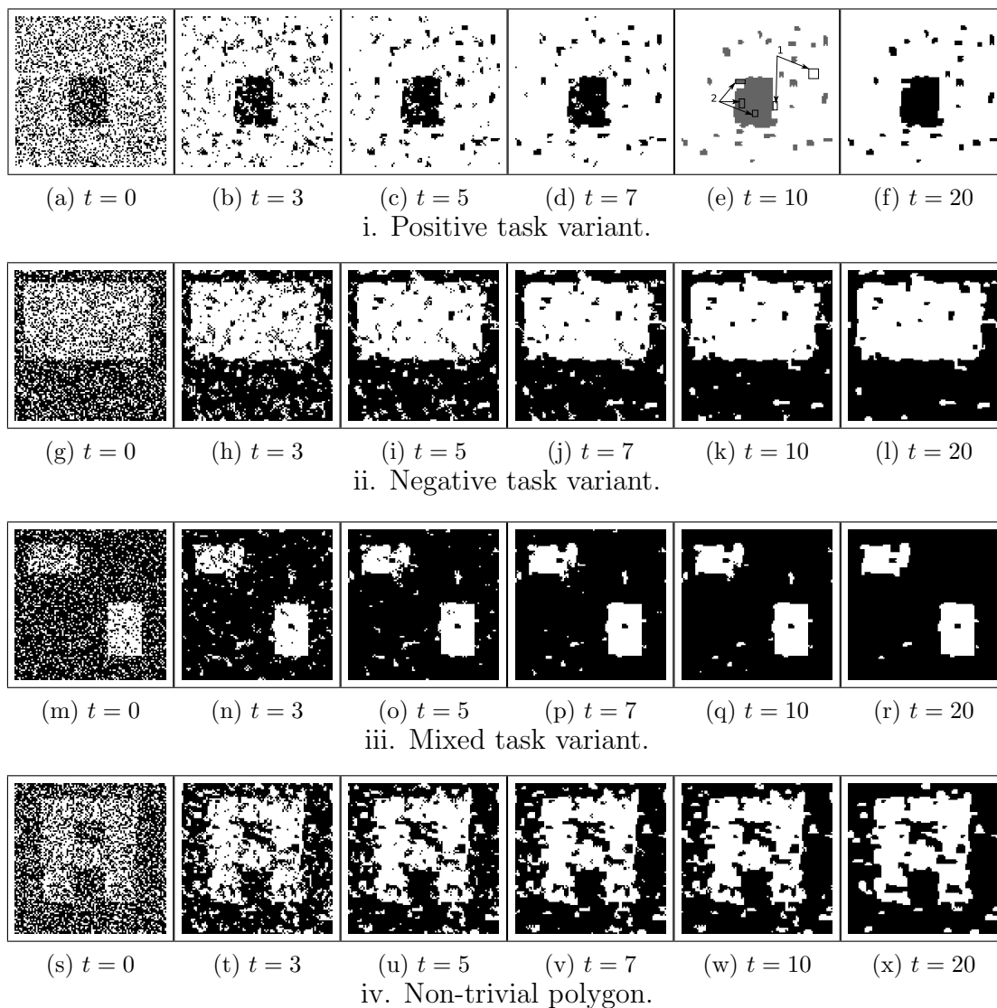
Figure 5.5: A series of space-time diagrams of a spatial density niching rule evolved by the genetic algorithm on 99 \times 99 lattice with r = 1 . (i.) Initial configuration for a positive task variant with a 67.87% density rectangle on a 38.11% background. (ii.) A negative task variant configuration with a 33.09% density rectangle in a foreground and a 68.06% density background. (iii.) Mixed niche variant with two rectangles of different densities. The top left quadrant of the lattice has a 19 \times 32 rectangle with density 49.51% and a 35 \times 22 rectangle with density 19.92% in the bottom right. (iv.) A solution for a non-trivial polygon. The ‘A’ shape foreground has a density 42.87% placed on the background with 65.46% density.
