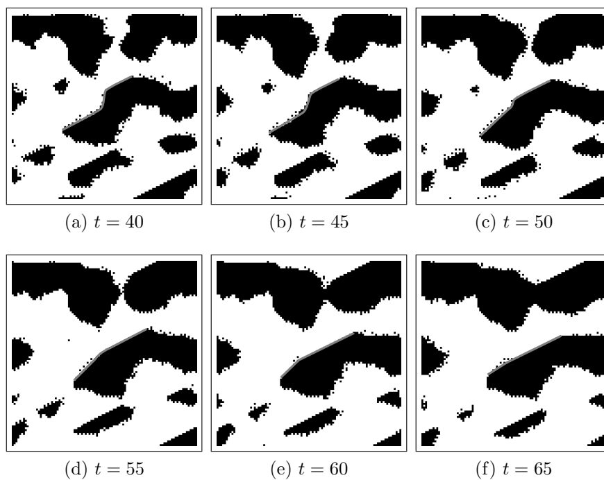
Figure 8.8: Cenek's rule for the two-dimensional density classification task. Lattice configurations are shown at times t = 40, 45, 50, 55, 60 , and 65 . A section of a black domain has a border marked with a gray line that suddenly reverses its direction of advancement, stops for several steps, and then starts moving again. This border region is located approximately in the middle of the highlighted domain border. The domain border was outlined manually.
